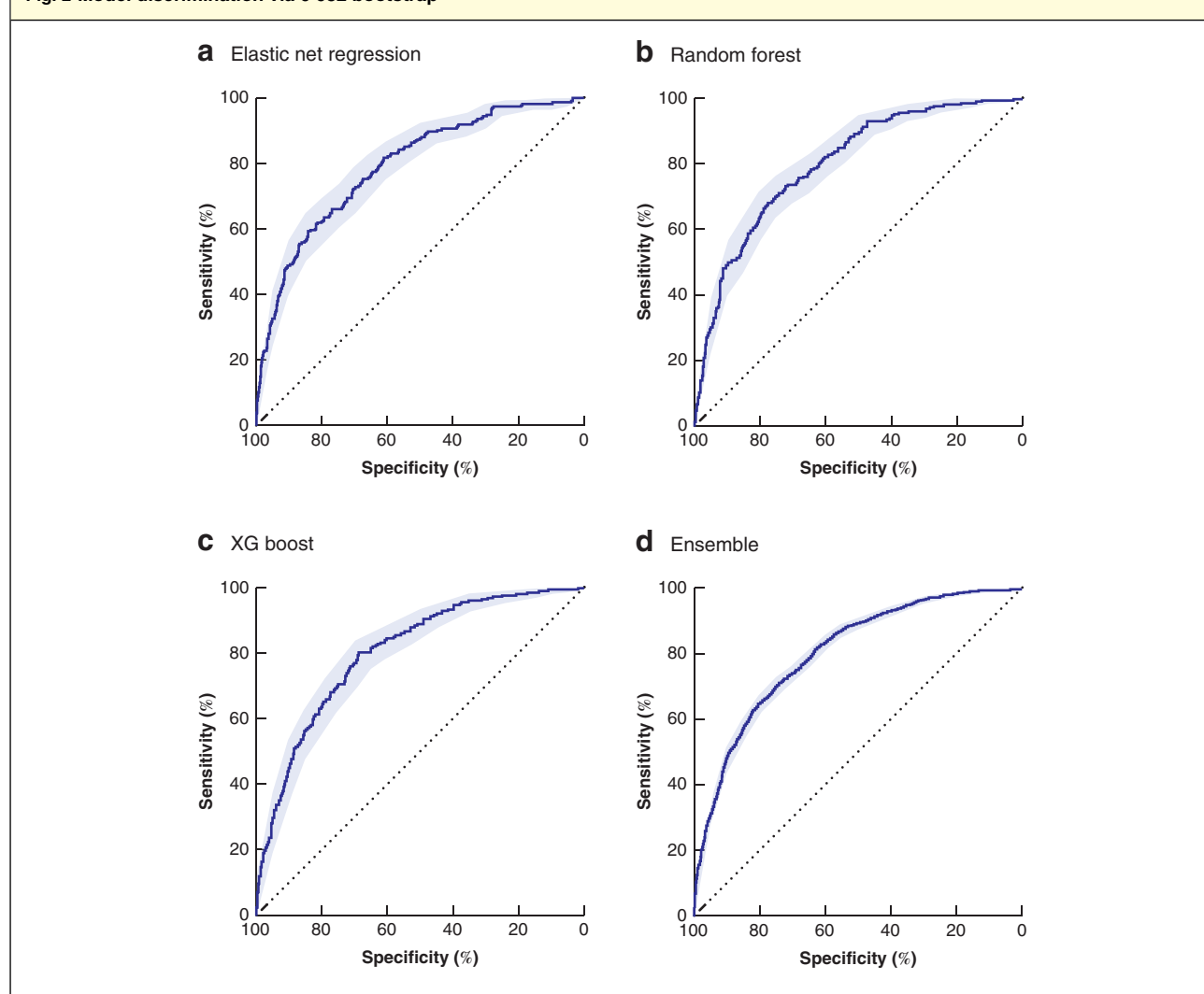
Fig. 2 Model discrimination via 0.632 bootstrap
