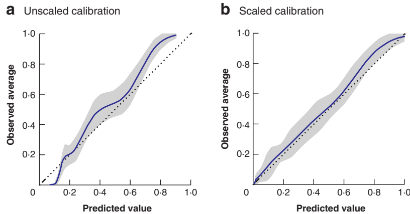
Fig. 3 Ensemble model calibration before and after adjustment
